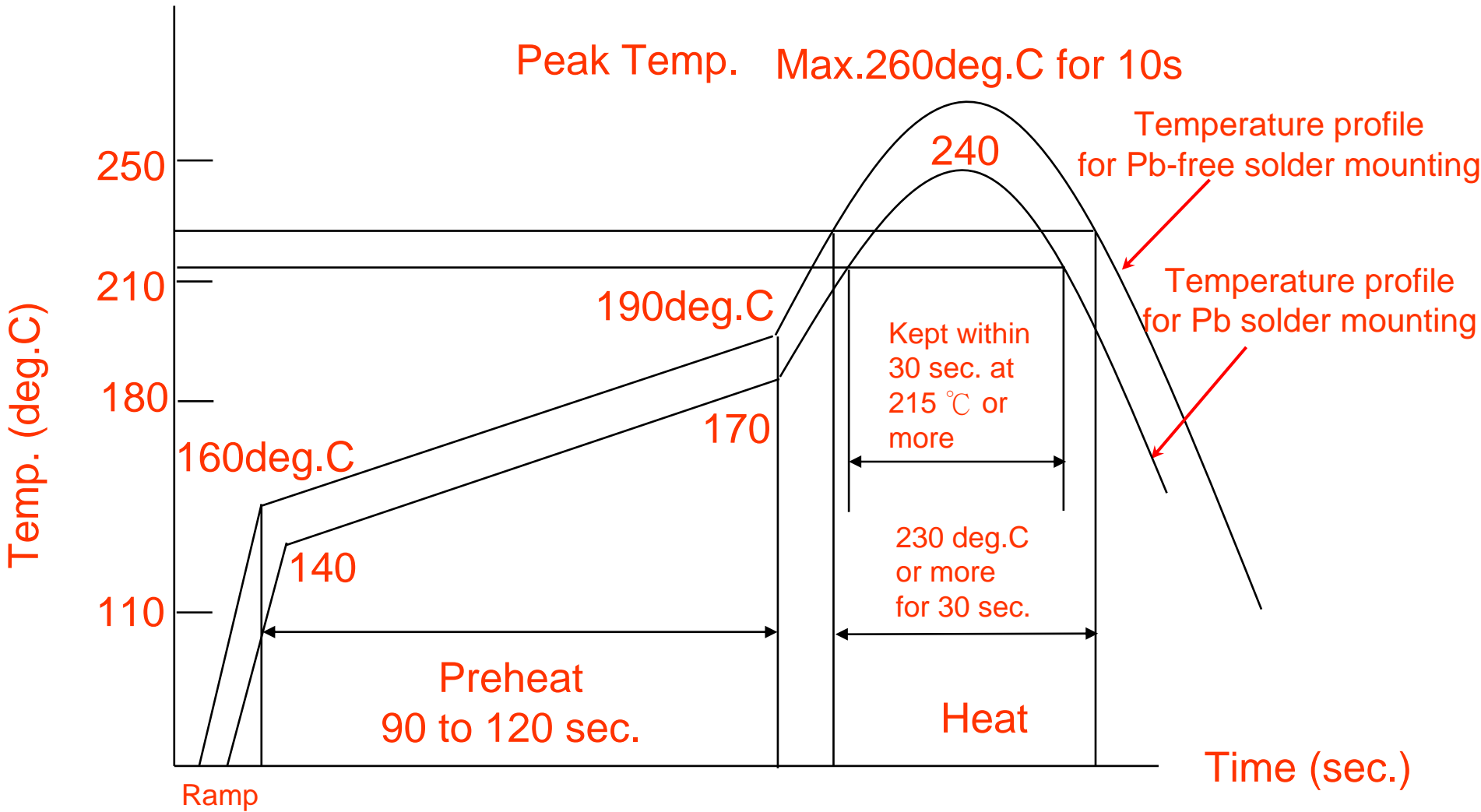
Standard Reflow Soldering Profile For SMD Devices
