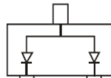
BAS40-06T Marking: 46
