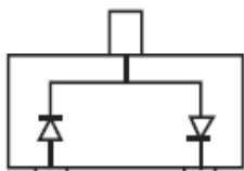
BAS40-04T Marking: 44
