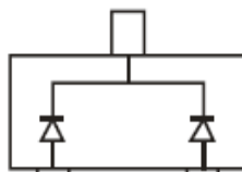
BAS40-05T Marking: 45
