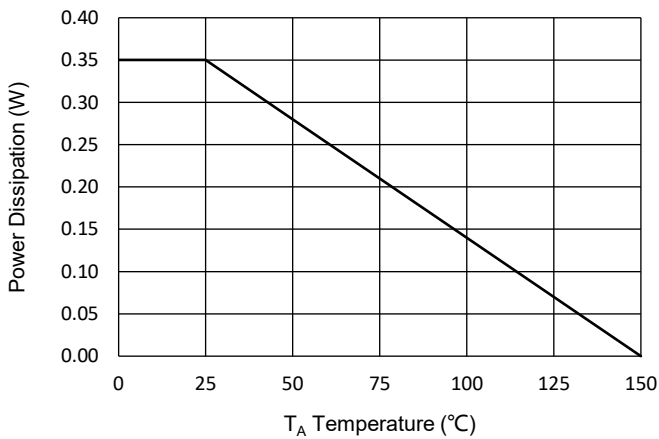
Fig.11 - PD Dissipation
