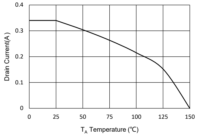
Fig.10 - Drain Current
