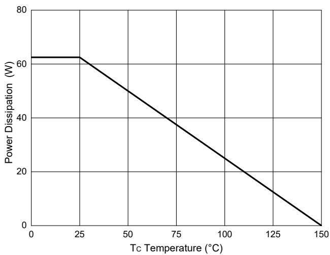
Fig.11-PD Dissipation
