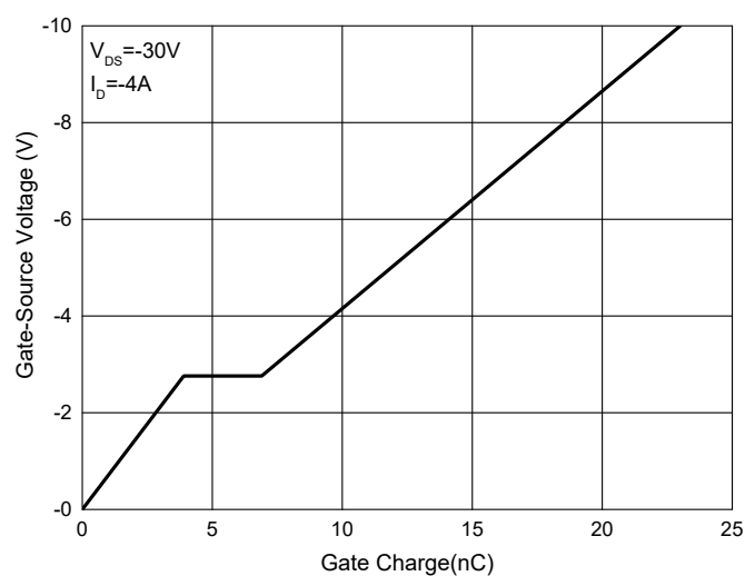
Fig. 8 - Gate Charge
