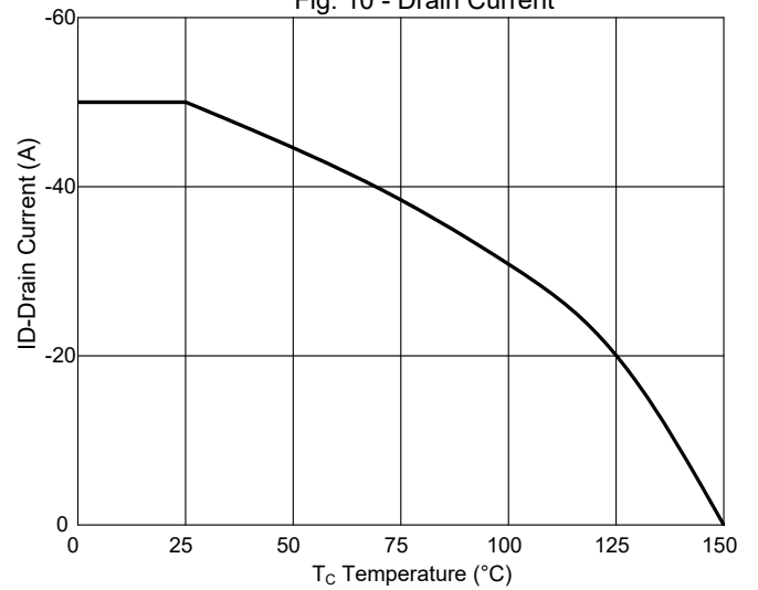
Fig. 10 - Drain Current
