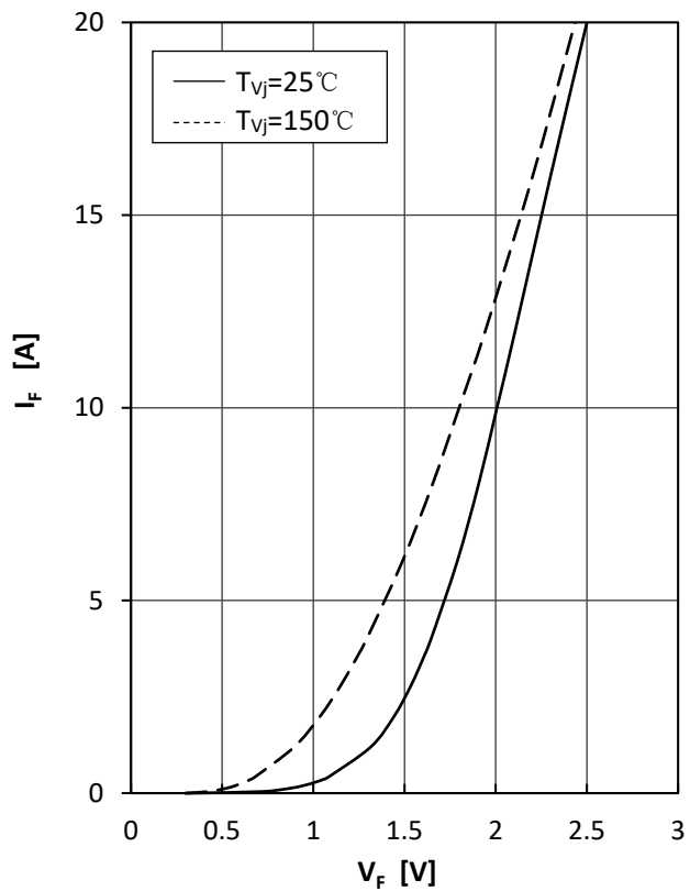
Fig13.Diode-brake-chopper Forward Characteristics
