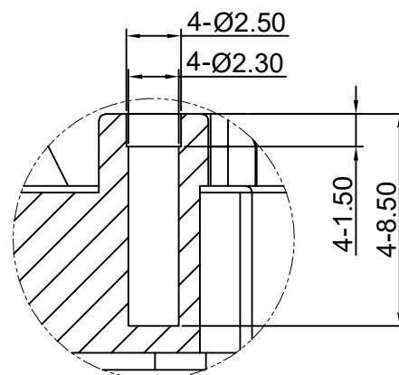
View C scale 4:1
