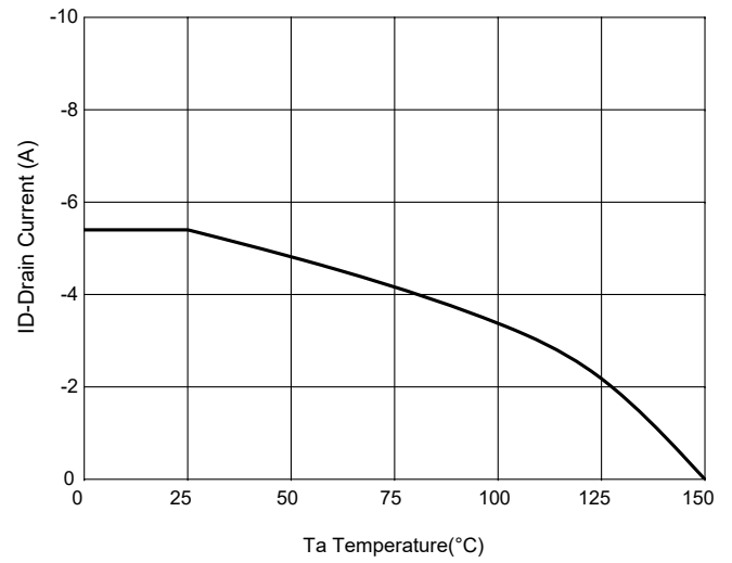
Fig. 10 - Current Dissipation
