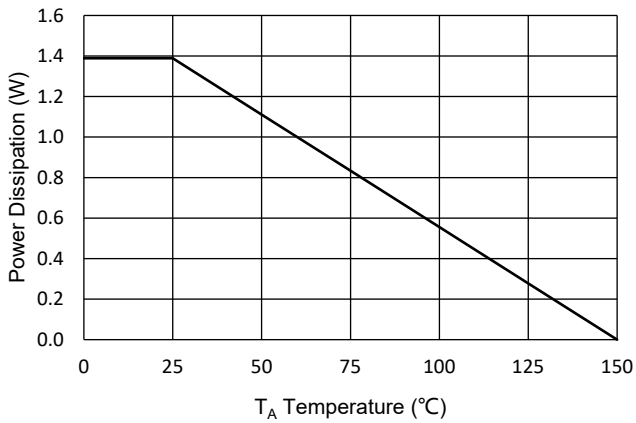
Fig.11 - PD Dissipation
