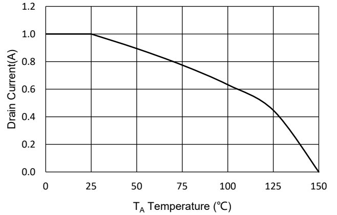
Fig.10 - Drain Current
