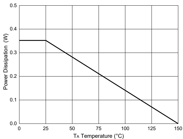
Fig.11 - PD Dissipation
