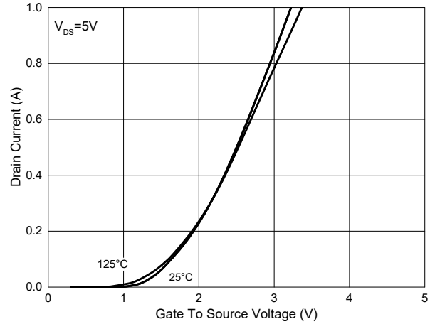
Fig.2 - Transfer Characteristic
