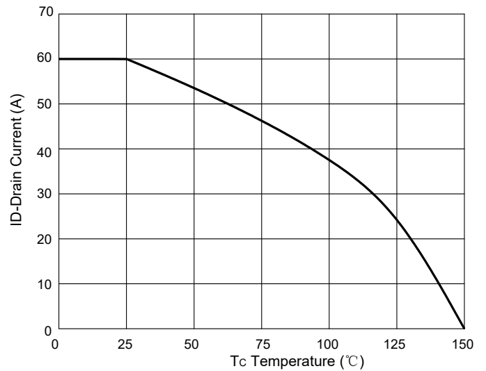
Fig. 10 - Drain Current
