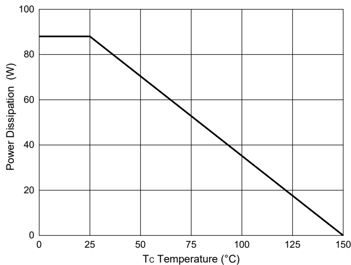
Fig.11-PD Dissipation
