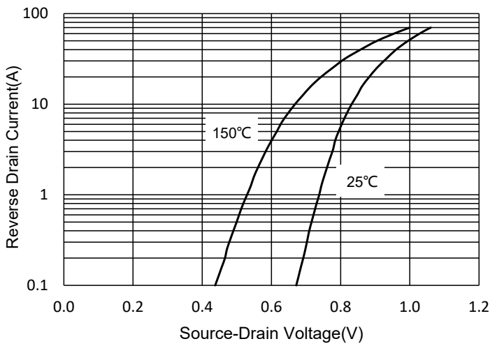
Fig.9 IS-VSD
