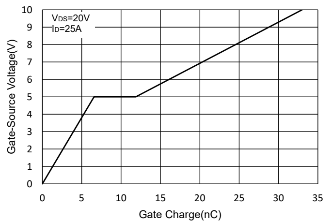
Fig.6 Gate Charge
