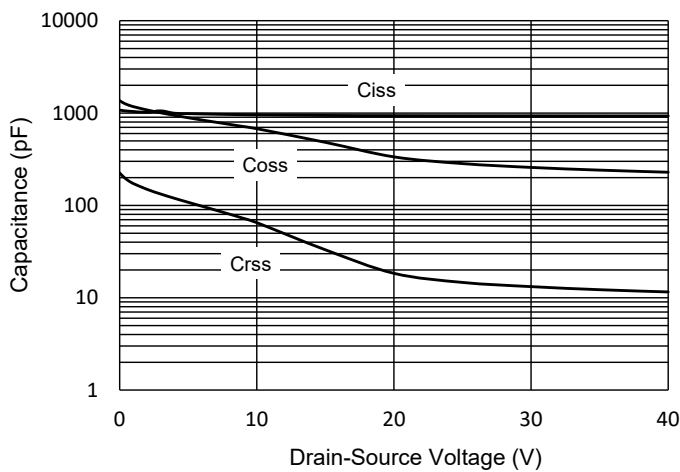
Fig.5 Capacitance Characteristics
