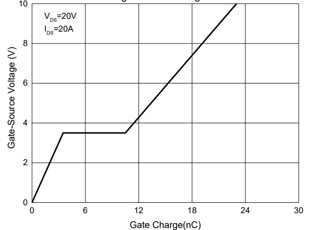
Fig. 6 - Gate Charge
