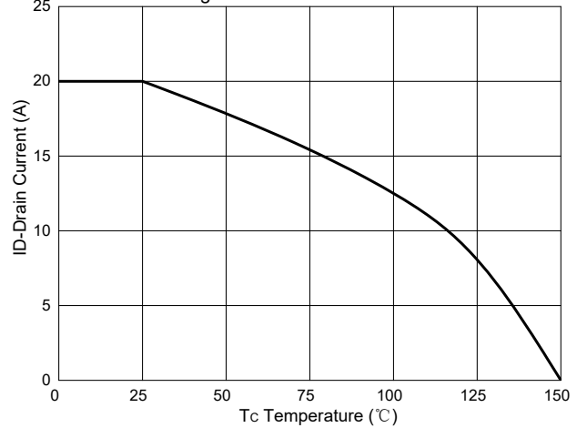
Fig. 10 - Drain Current
