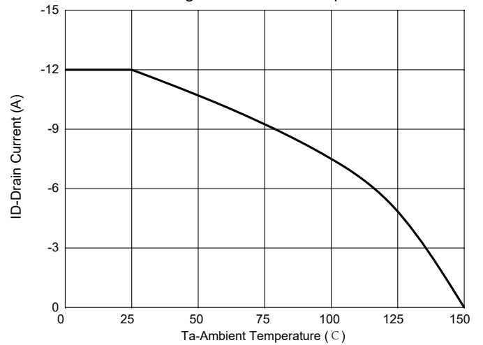
Fig. 10 - Current Dissipation
