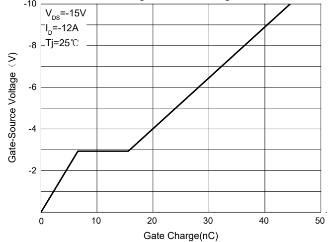
Fig. 6 - Gate Charge
