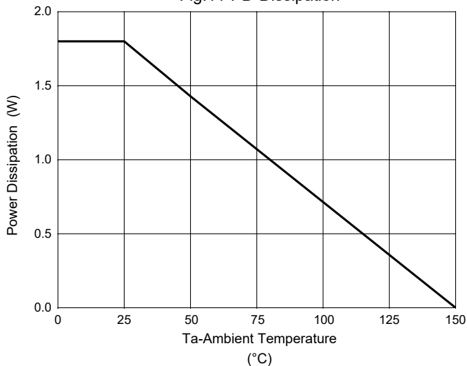
Fig.11-PD-Dissipation
