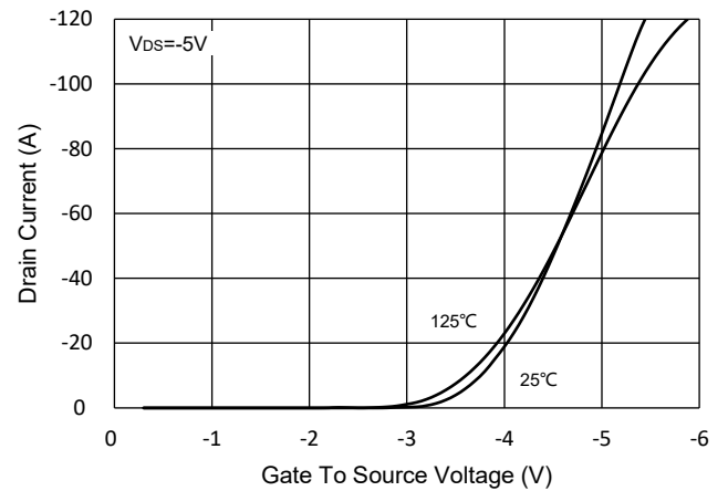
Fig.2 - Transfer Characteristic
