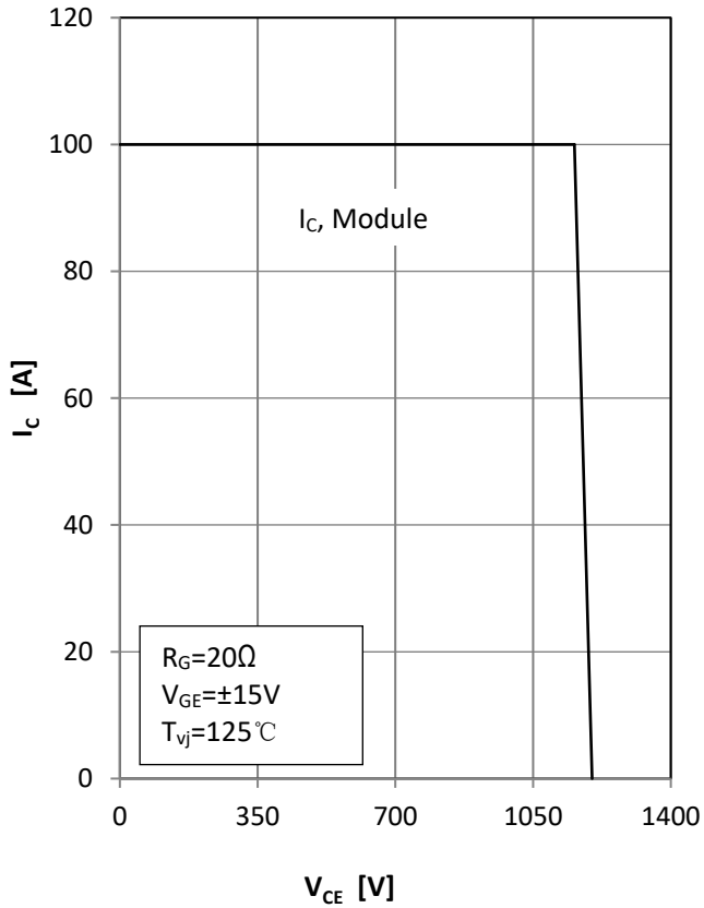
Fig5. RBSOA
