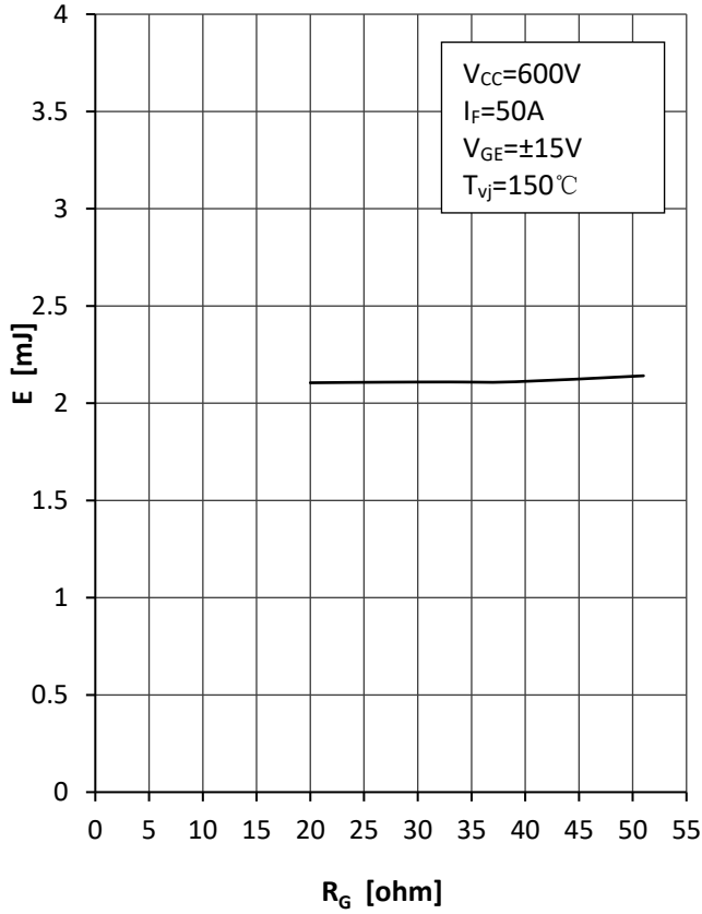
Fig9.Diode Switching Loss vs.Rg
