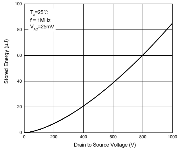
Fig. 12 - Output Capacitor Stored Energy
